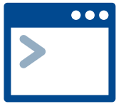
Command Line
